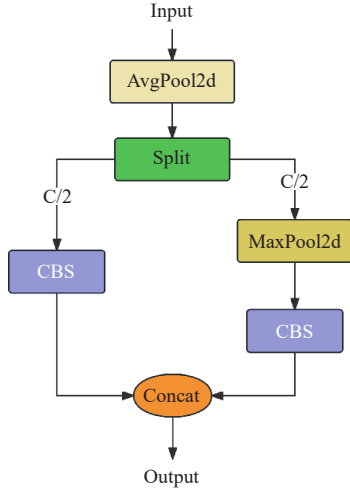
Figure 5 Structure of ADown module
