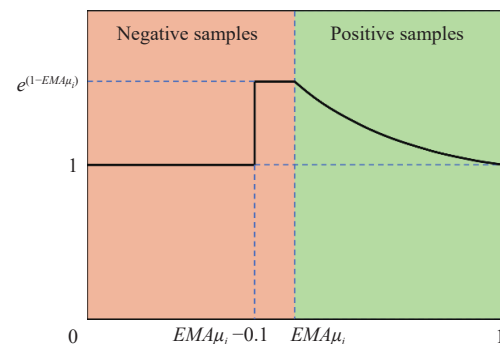
Figure 8 EMA-Slide Loss
