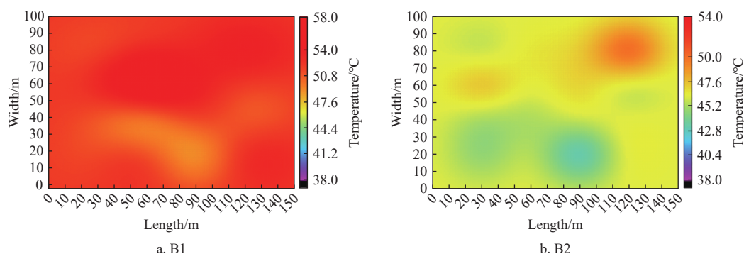
Figure 12 Indoor air temperature of different single-ventilation areas after 1 h of ventilation
