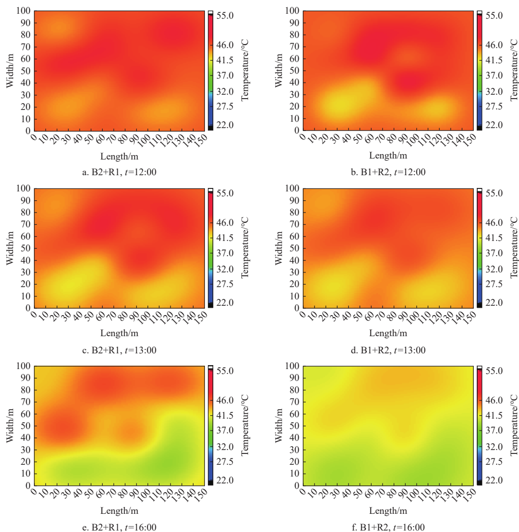
Figure 16 Indoor temperature cloud map at different moments after ventilation under B2+R1 and B1+R2 conditions
