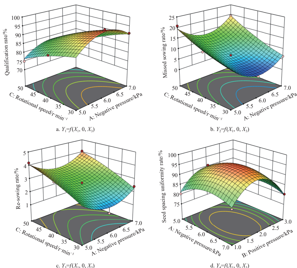
Figure 12 Response surface plots of the evaluation indices
