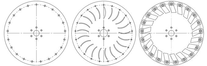
Figure 3 Different specifications of seed-metering discs
