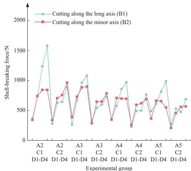
Figure 9 Statistical diagram of the impact of cutting direction on compressive mechanical properties
