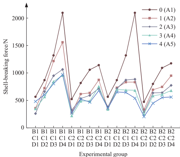
Figure 8 Statistical diagram of the effect of the number of cutting knives on compressive mechanical properties
