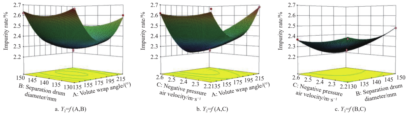
Figure 10 3D surface plots showing the effects of different factors on the impurity rate
