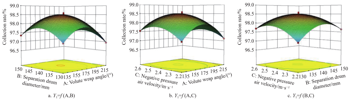
Figure 9 3D surface plots showing the effects of different factors on the collection rate
