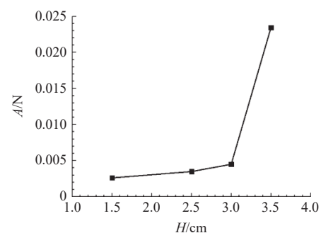
Figure 5 Drag force amplitude of the rice seedling under different wave heights for \lambda=35 cm
