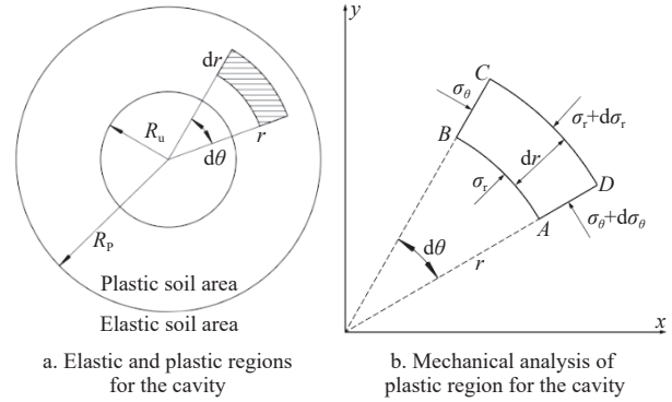
Figure 6 Detailed analysis of both elastic and plastic regions along with the corresponding stress states for the cavity system
