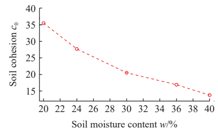
Figure 11 Variation trend in the in-situ soil cohesion across a soil moisture content range of 20% to 40%
