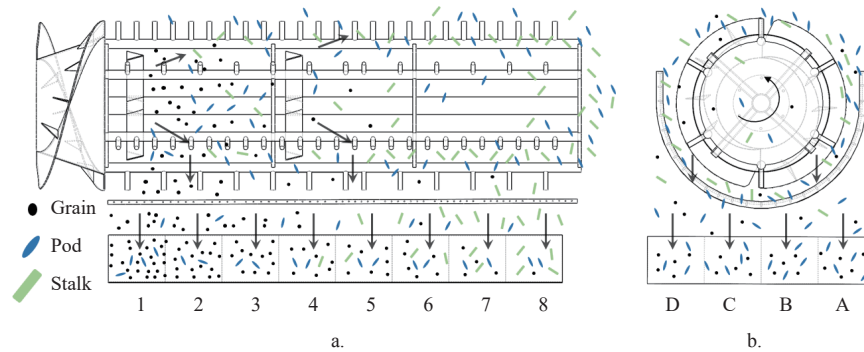
Figure 2 Working process of the pneumatic-assisted threshing-separation device
