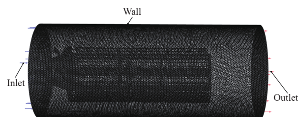
Figure 6 Mesh generation of the computational domain
