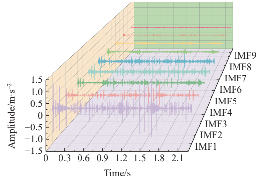
Figure 9 IMF components obtained by EEMD
