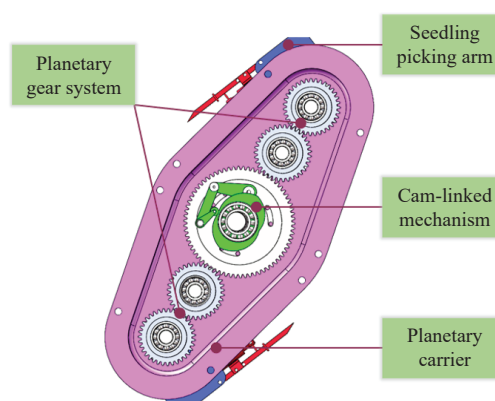
b. The cam-linked planetary gear system automatic seedling picking mechanism
