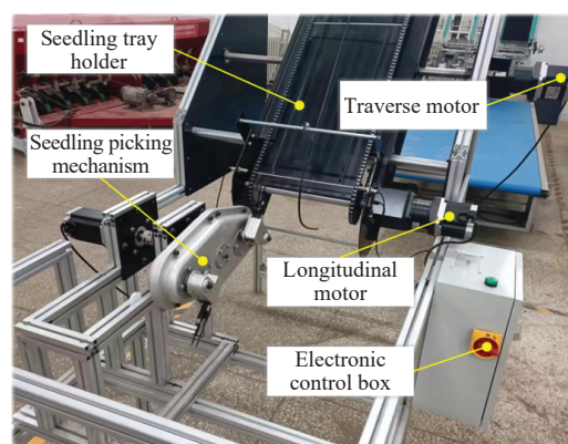
a. The automatic vegetable transplanting machine test bench
