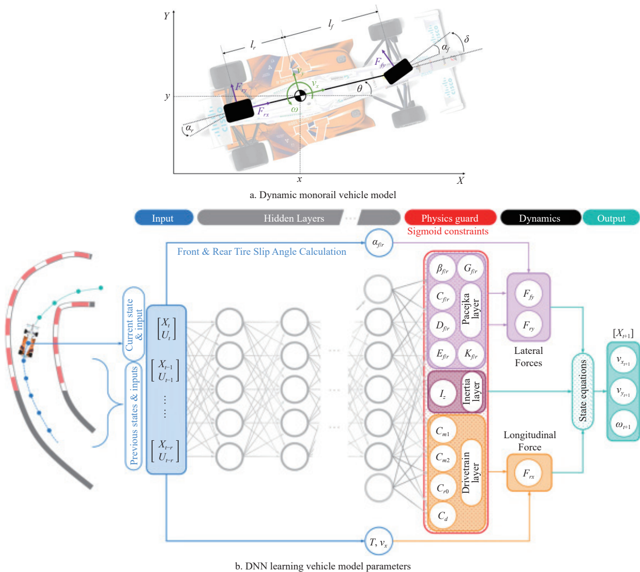
Figure 6 Physics-constrained neural network (PCNN) for vehicle dynamics modeling
