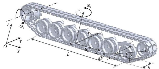
Figure 3 Single track motions on terrain and forces and
