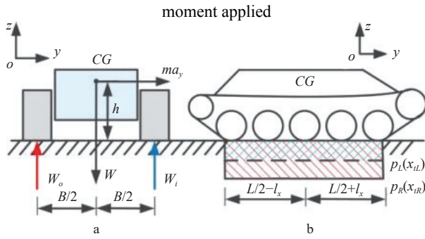
Figure 4 Normal pressure distribution on the track-ground interface
