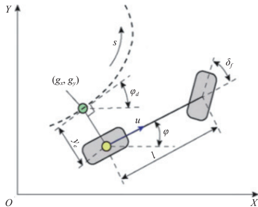
Figure 9 Path-tracking control based on kinematics model
