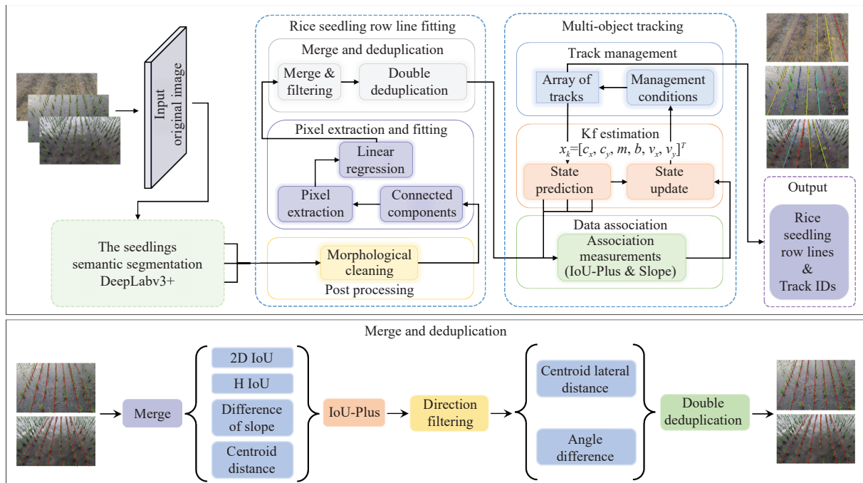
Figure 3 Framework of the proposed RTrack-DL model
