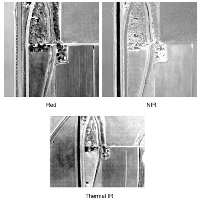
Figure 10 TTAMRSS images over a canal section
