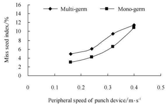
Figure 7 Effect of feeding disc peripheral speed on the seed miss index
