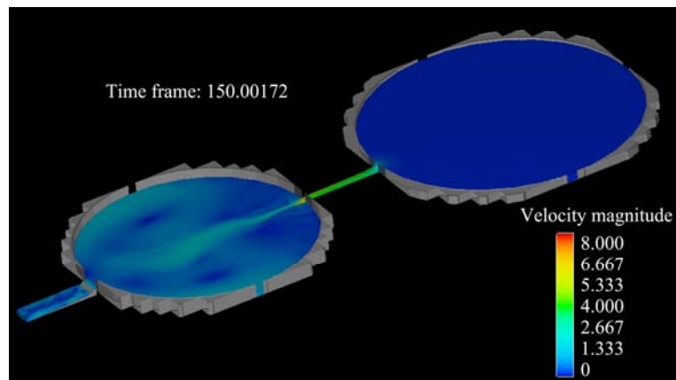
Figure 4 Fluid velocity distribution of the entire domain at 150 s in case I
