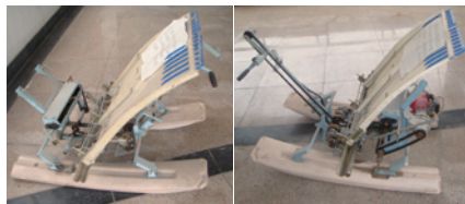
The manufactured two kinds of "Yulong" hill-type rice transplanters after transferring patents and technologies. (Photographs of two types)
