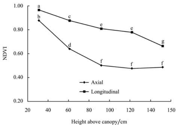
Figure 3 Response of reflectance values to height above target and orientation of the window boxes relative to the sensor head.
