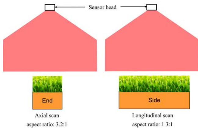
Figure 2 GreenSeeker handheld optical sensor passed at two different angles relative to window boxes planted with ryegrass to determine the effect of orientation on NDVI. Aspect ratio was calculated as the ratio between the GreenSeeker light beam width (61 cm) and the traversed width of the planter box (19.1 cm for axial scan and 45.7 cm for longitudinal scan). Shape of light pattern is author's conceptual depiction based on available information
