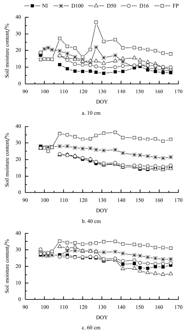
Figure 3 Volumetric soil moisture content in different treatments on day of year (DOY) at three different soil depths
