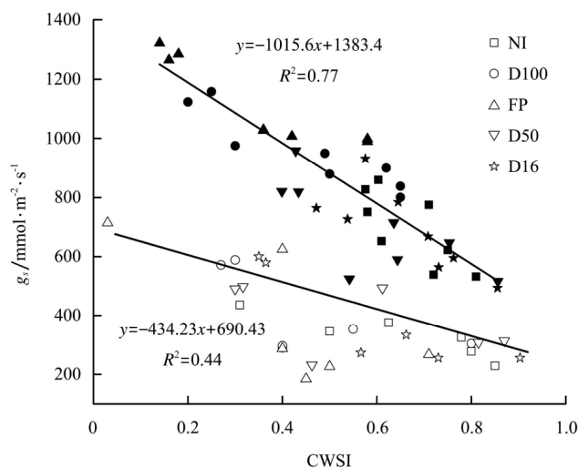
Figure 6 Correlation between CWSI and stomatal conductance ( g_s ) at pre-heading (hollow data points) and post-heading stage (filled data points) for the different treatments
