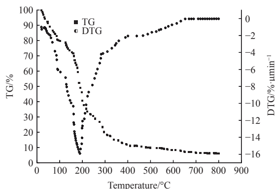
a. TG and DTG curves of tar obtained with 10 °C/min
