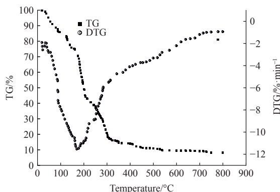
b. TG and DTG curves of tar obtained with 20 °C/min
