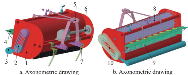
1. Chopping chamber, 2. Decelerating device, 3. Depth limiting device, 4. Spreading device for chopped stalk, 5. Suspension device, 6. Transmission device, 7. Provoking device for maize stalk, 8. Sliding-supporting device, 9. Collecting-chopping device, 10. Accelerating device
