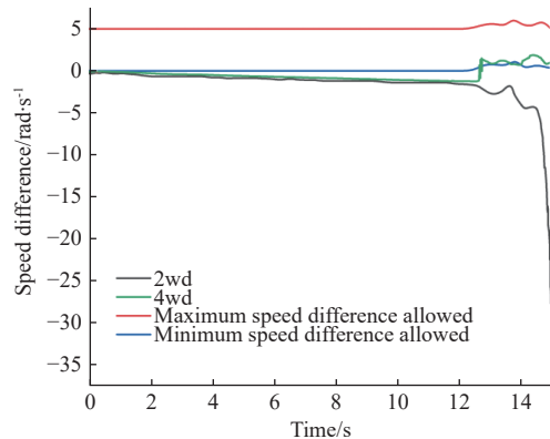
b. Front and rear axle speed difference
