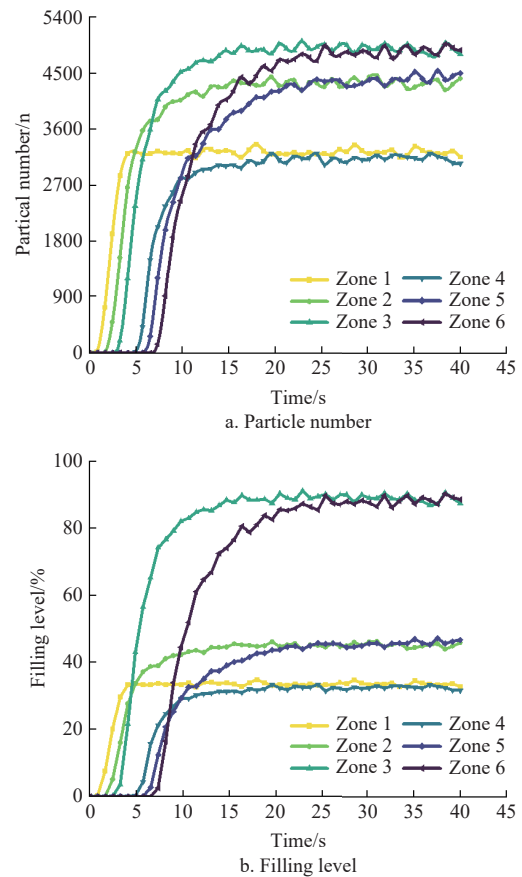
Figure 7 Variation of particle number and filling level in different regions over time
