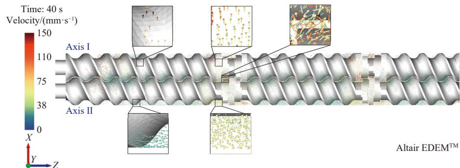
Figure 13 Direction of motion of simulated particles at 40 s
