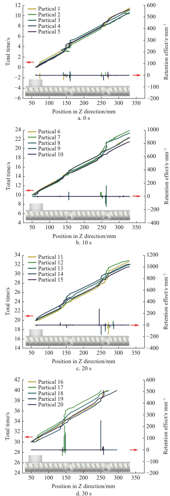
Figure 8 Displacement-time relationship of particles entering the barrel at different times
