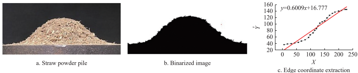
Figure 1 Angle of repose processing image
