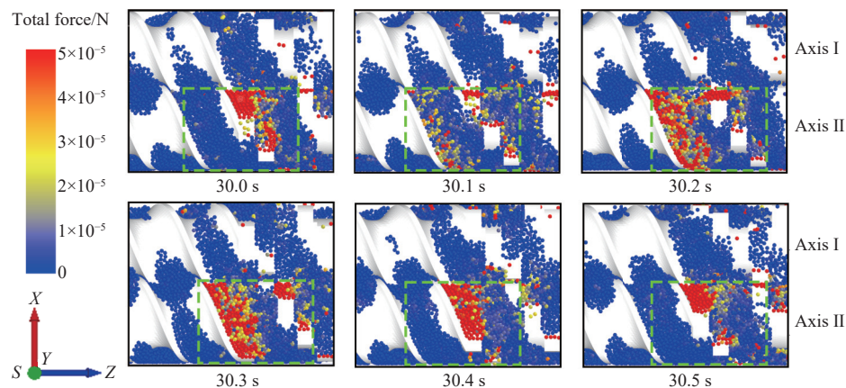
Figure 12 Variation of force with time for simulated particles of Zones 1 and 3
