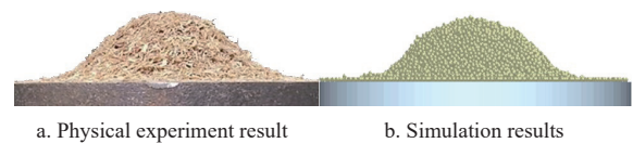
Figure 4 Comparison of physical experiment and simulation results
