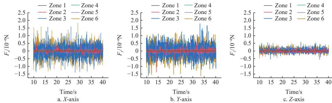
Figure 11 Variation of simulated particle forces along different directions
