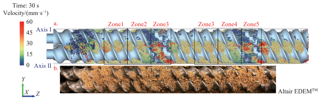
Figure 5 Comparison between simulation and actual results
