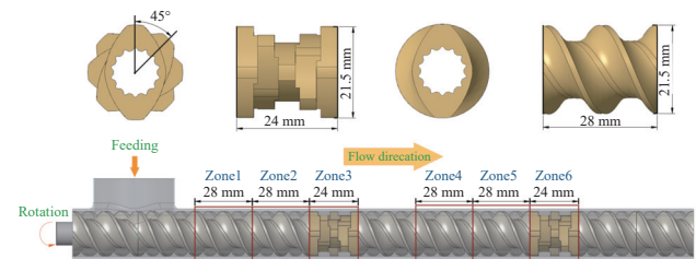
Figure 2 Schematic diagram of computational domain division
