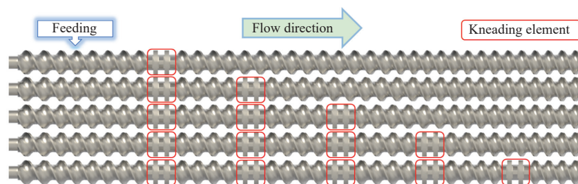
Figure 3 Configuration of screws
