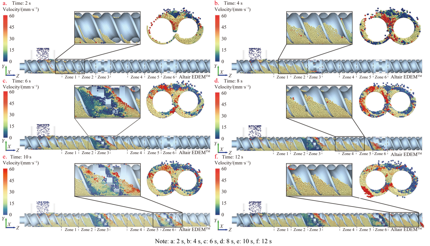
Figure 10 Simulated particle distribution at different time points
