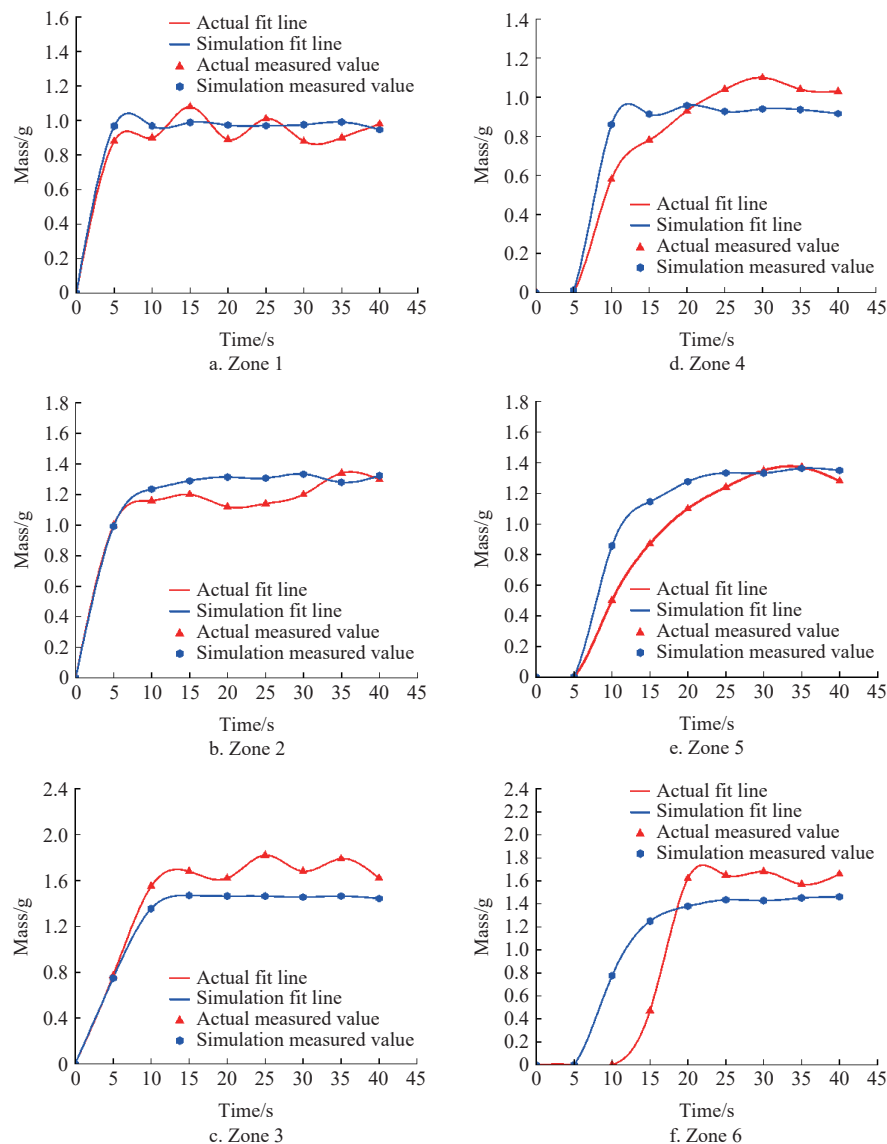
Figure 6 Variation of particle mass in different zones over time during simulation experiment and physical experiment
