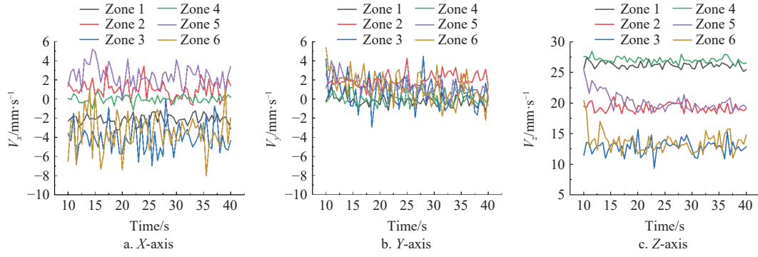
Figure 9 Variation of simulated particle velocity along different directions
