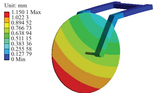
Figure 13 Cloud diagram of total deformation of grass roller
