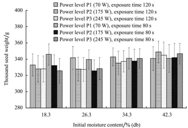
Figure 8 Thousand grain weight of corn at different initial moisture content dried with microwave
